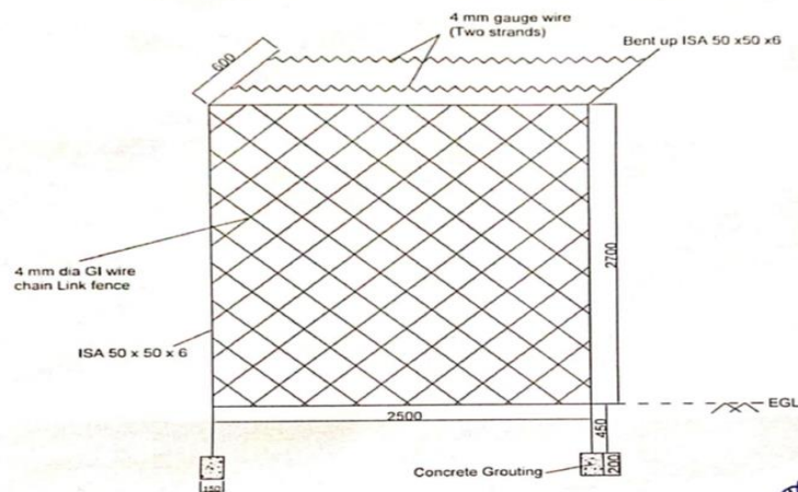
Fig : A typical section of fencing between two ISA Column Note : All dimensions are in "mm" unless otherwise specified. Total Length of fencing = 3500 Meter.
